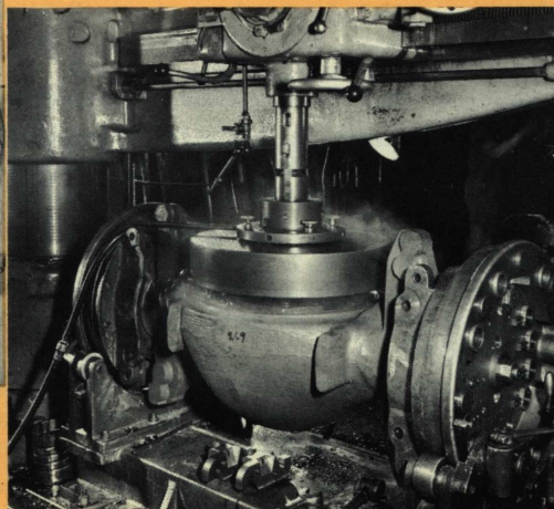
Boring "banjo" housing. Here is a job that proves a radial-boring 19 \frac{1}{2} " diameter in cast steel differential housings on a production-line basis. Chipmaster radials also are used for drilling, tapping, and facing these parts.
