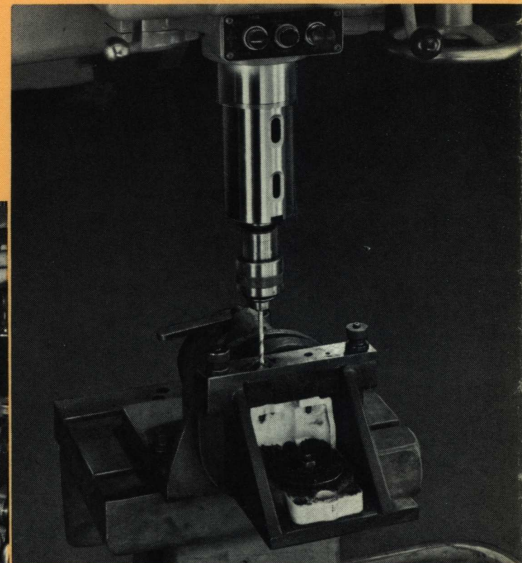
Small-hole drilling and tapping. The same Chipmaster that handles heavier jobs than any other radial is an accurate, sensitive machine that handles \frac{3}{16} " and \frac{1}{4} " drills and taps at high speeds.
